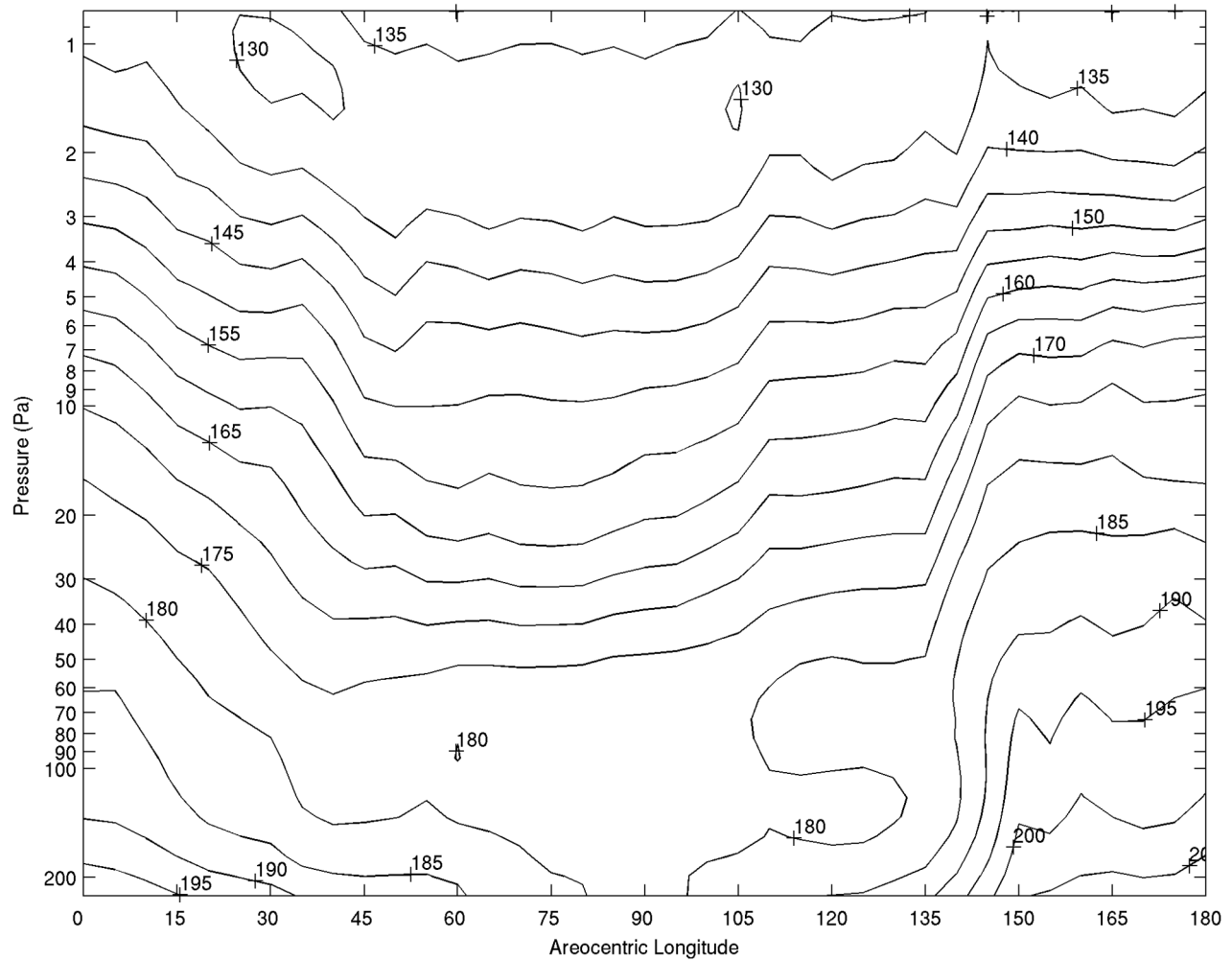
Figure 9. Zonal average nightside temperature (K) between 5^{\circ} S and 5^{\circ} N, L_s = 0^{\circ} – 180^{\circ} for MY 29. The pressure range is restricted for emphasis.
