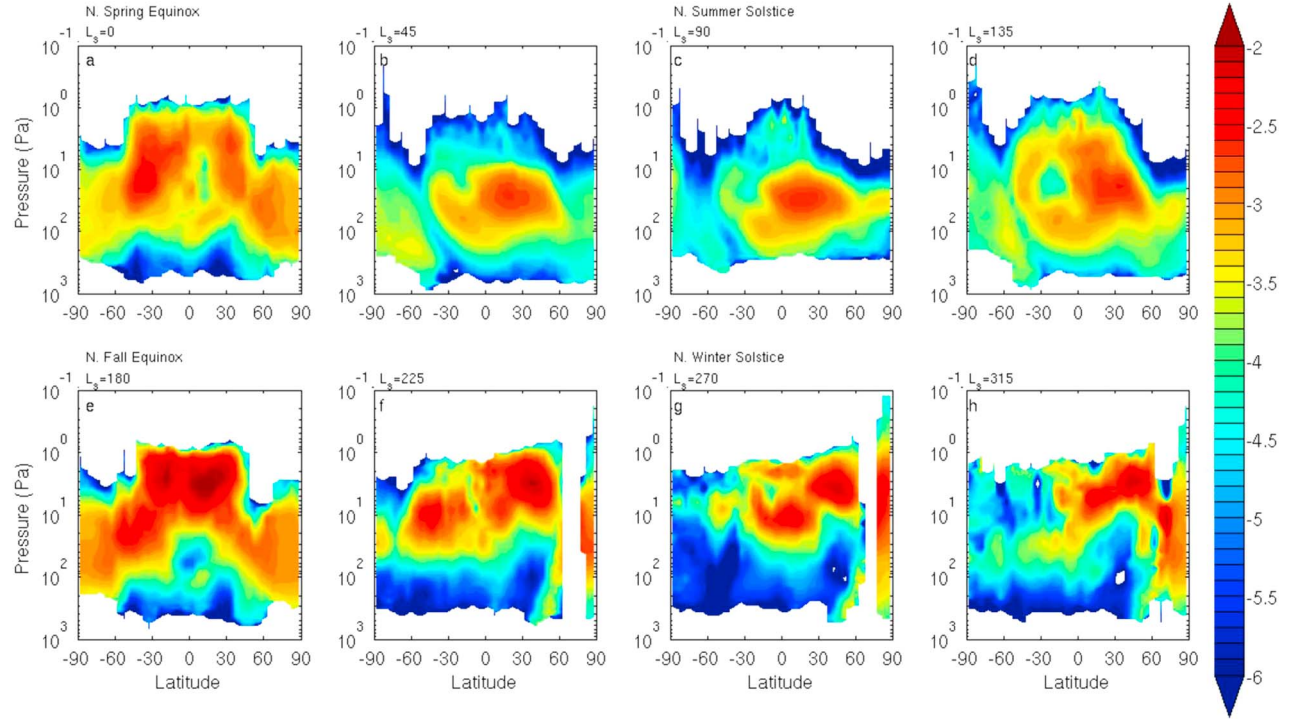
Figure 16. \text{Log}_{10} of the zonal average water ice density-scaled opacity ( \text{m}^2 \text{kg}^{-1} ) nightside retrievals for MY 29 for the L_s bins labeled at the top of each panel. Contours are shown every 0.1 log units. Note the pressure scale is between 1000 and 0.1 Pa.
