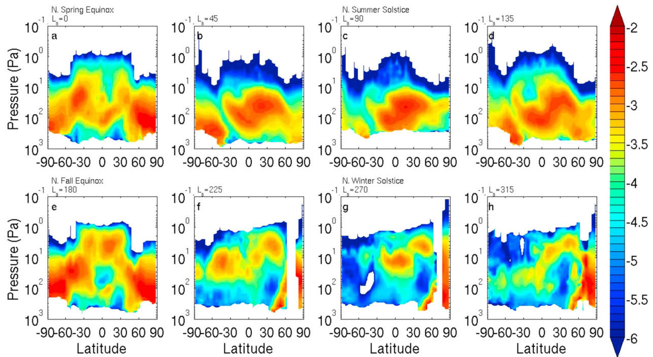
Figure 18. \log_{10} of the zonal average water ice opacity ( \text{km}^{-1} ) nightside retrievals of MY 29 for the L_s bins labeled at the top of each panel. Contours are shown every 0.1 log units. Note the pressure scale is between 1000 and 0.1 Pa.
