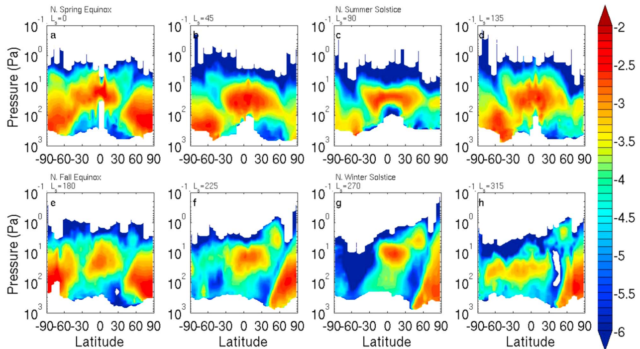
Figure 19. \log_{10} of the zonal average water ice opacity ( \text{km}^{-1} ) dayside retrievals of MY 29 for the L_s bins labeled at the top of each panel. Contours are shown every 0.1 log units. Note the pressure scale is between 1000 and 0.1 Pa.
