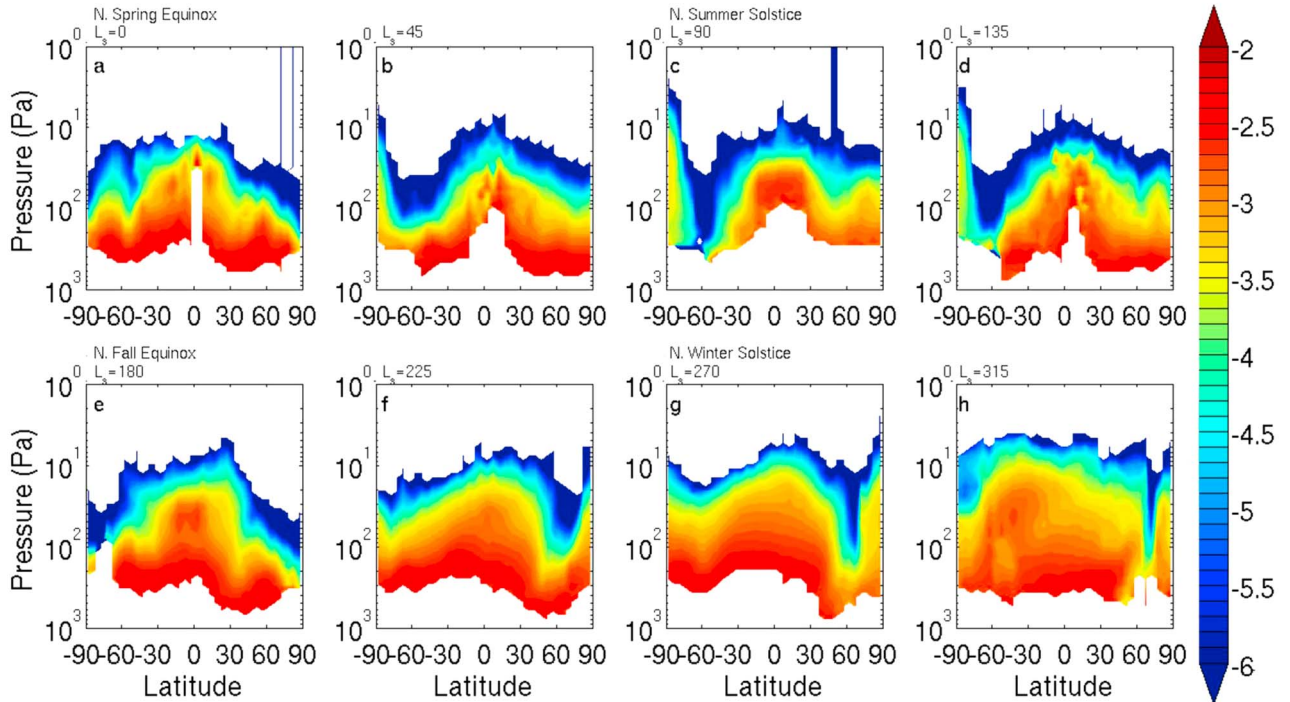
Figure 13. \log_{10} of the zonal average dust opacity ( \text{km}^{-1} ) dayside retrievals of MY 29 for the L_s bins labeled at the top of each panel. Contours are shown every 0.1 log units. Note the pressure scale is between 1000 and 1 Pa.
