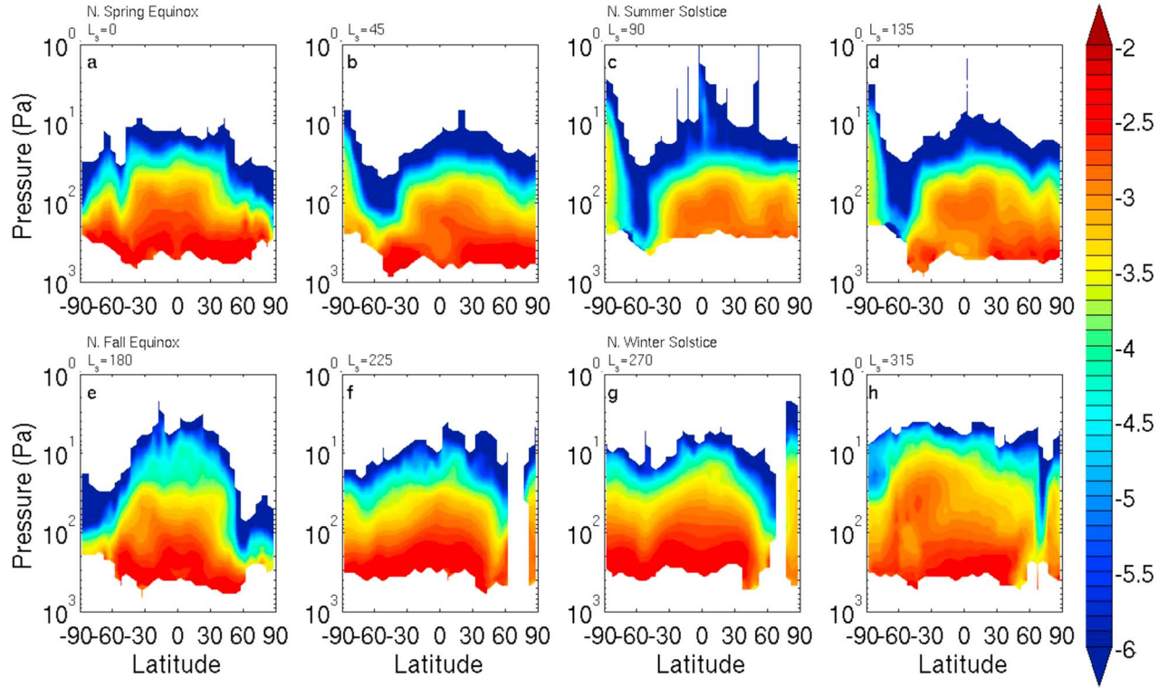
Figure 12. \log_{10} of the zonal average dust opacity ( \text{km}^{-1} ) nightside retrievals of MY 29 for the L_s bins labeled at the top of each panel. Contours are shown every 0.1 log units. Note the pressure scale is between 1000 and 1 Pa.
